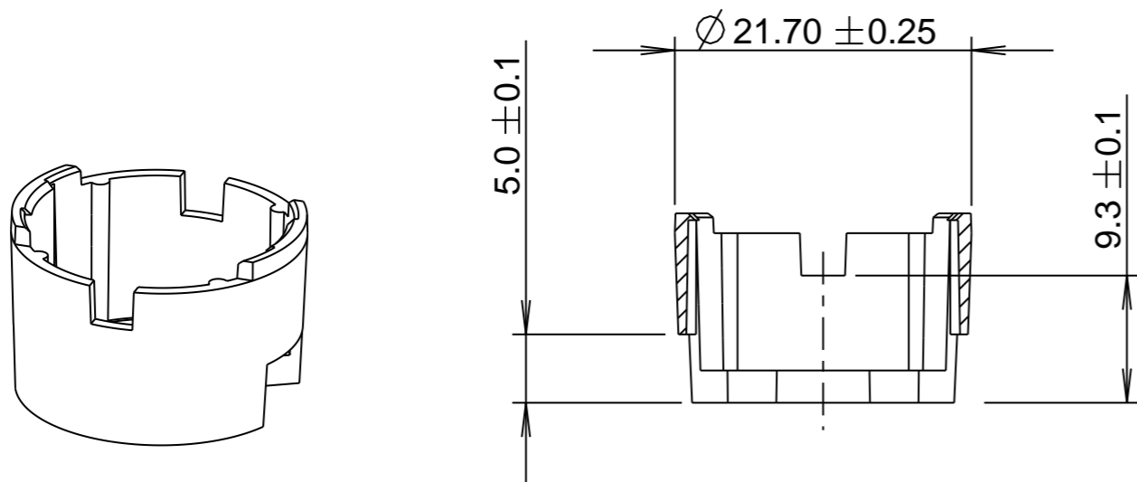
SECTION X-X
